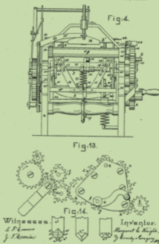
M. E. KNIGHT. Paper-Bag Machine. No. 220,925. Patented Oct. 28, 1879.
