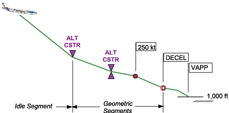
FMGS Descent Profile
