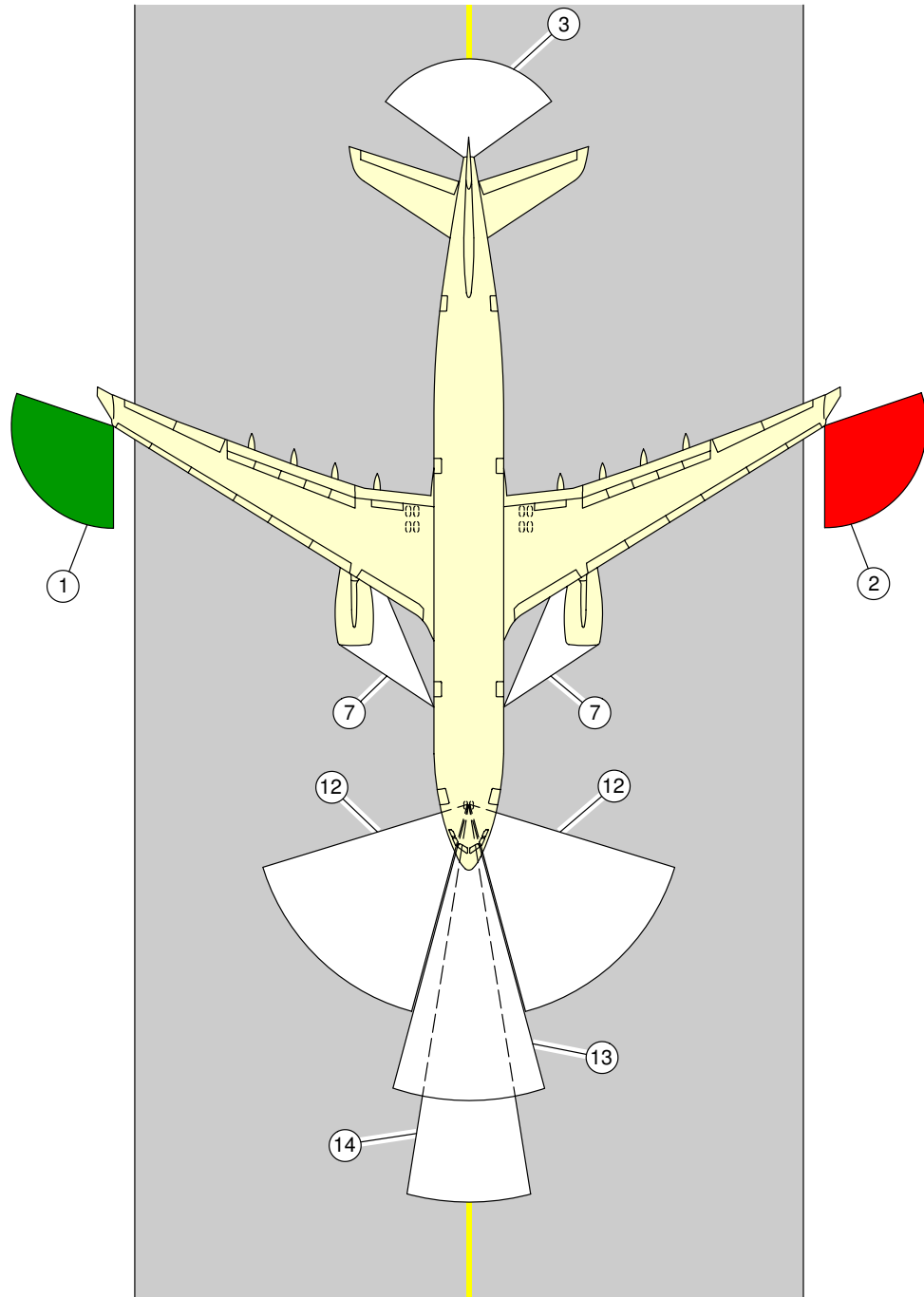
Exterior Lighting (Sheet 3 of 5) FIGURE-2-10-0-991-001-A01
